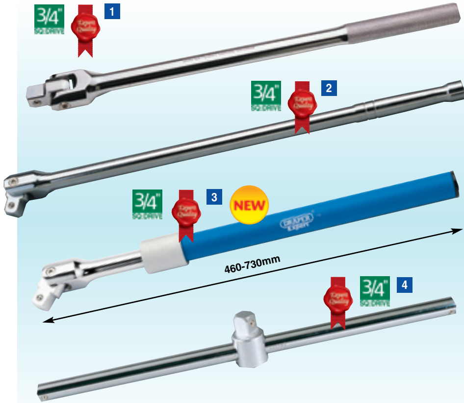
1 T12 3/4" Sq. Dr. 475mm Flexible Handle
