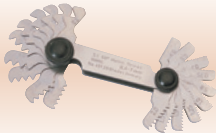
4 401 20 Blade Metric Screwpitch Gauge Set
