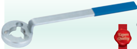
1 WPW-AC1 300mm VW/Audi Waterpump Pulley Locking Wrench for Air Conditioned Vehicles
